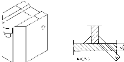
Filled weld
