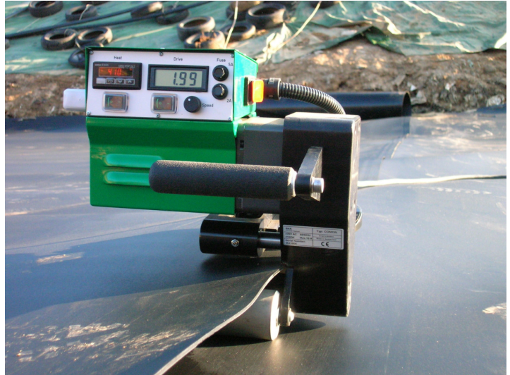
Techspan heavy duty wedge welder type 'Comon' with optional ceramic wedge
